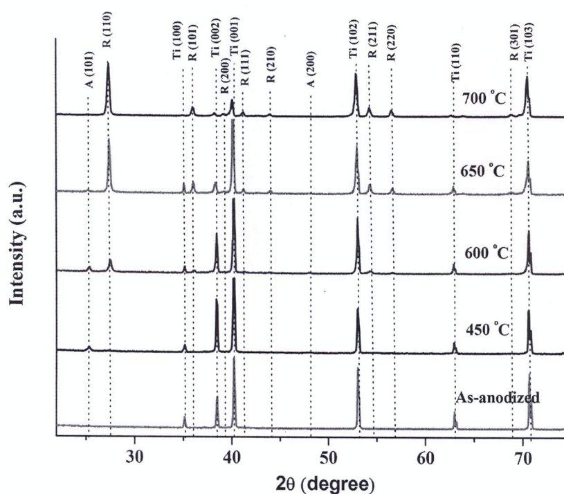
Fig. 2. XRD patterns of the as-anodized and sintered \text{TiO}_2 nanotubes (A-anatase, R-rutile, Ti-titanium).
