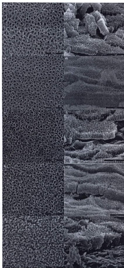
Fig. 1. SEM micrographs of the top and side views of \text{TiO}_2 nanotubes sintered at different temperatures: (a and b) as-anodized, (c and d) 450^\circ\text{C} , (e and f) 600^\circ\text{C} , (g and h) 650^\circ\text{C} , (i and j) 700^\circ\text{C} .
