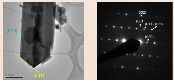
TEM image of typical Na 0.76 Fe 0.79 Ti 1.21 O 4 crystal and corresponding SEAD pattern
