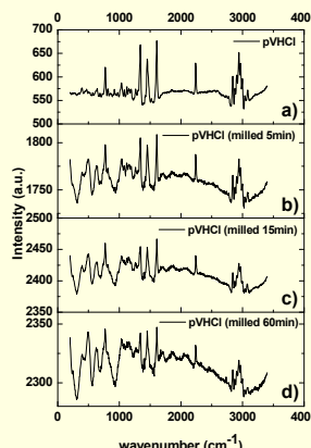
Fig. 6. Raman spectra of mechanically activated a) pVHCl milled for b) 5 min, c) 15 min and d) 60 min.
