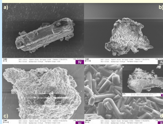
Fig. 3. Scanning electron micrographs of a) pVHCl milled for b) 5 min, c) 15 min and d) 60 min.
